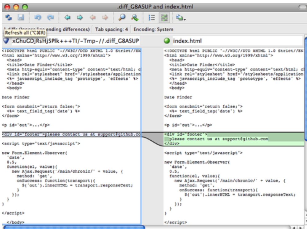
Figure 142. P4Merge.
